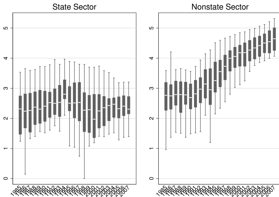
Figure 1: Box Plot of Total Factor Productivity
